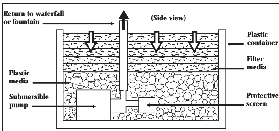
Figure 1. In-pond mechanical/bio-filter.
